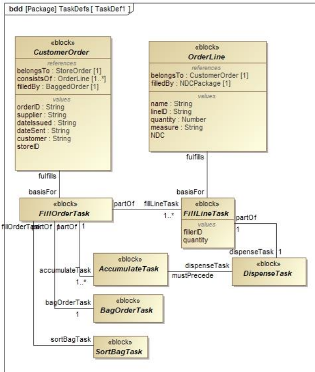
Figure 5-10 Task Structure for CFP
