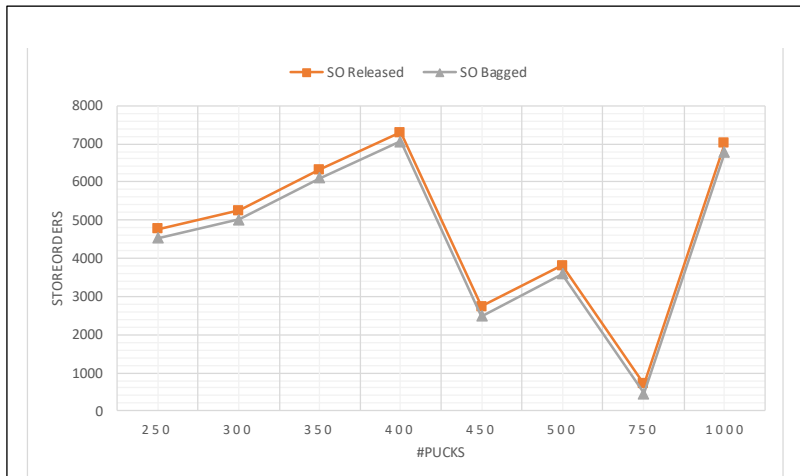
Figure 7-13 Throughput vs Number of Pucks; 250 Totes
