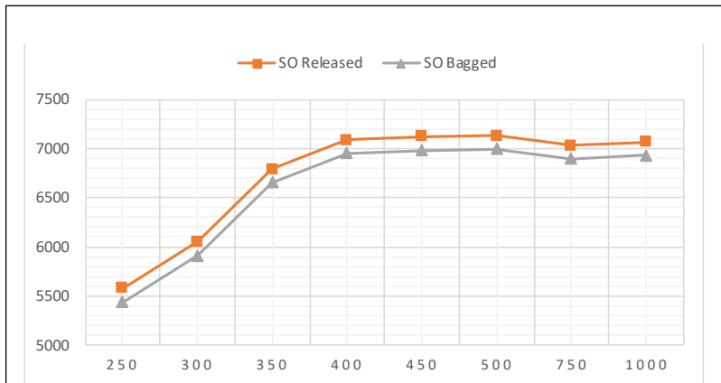
Figure 7-12 Throughput vs Number of Pucks; 200 Totes
